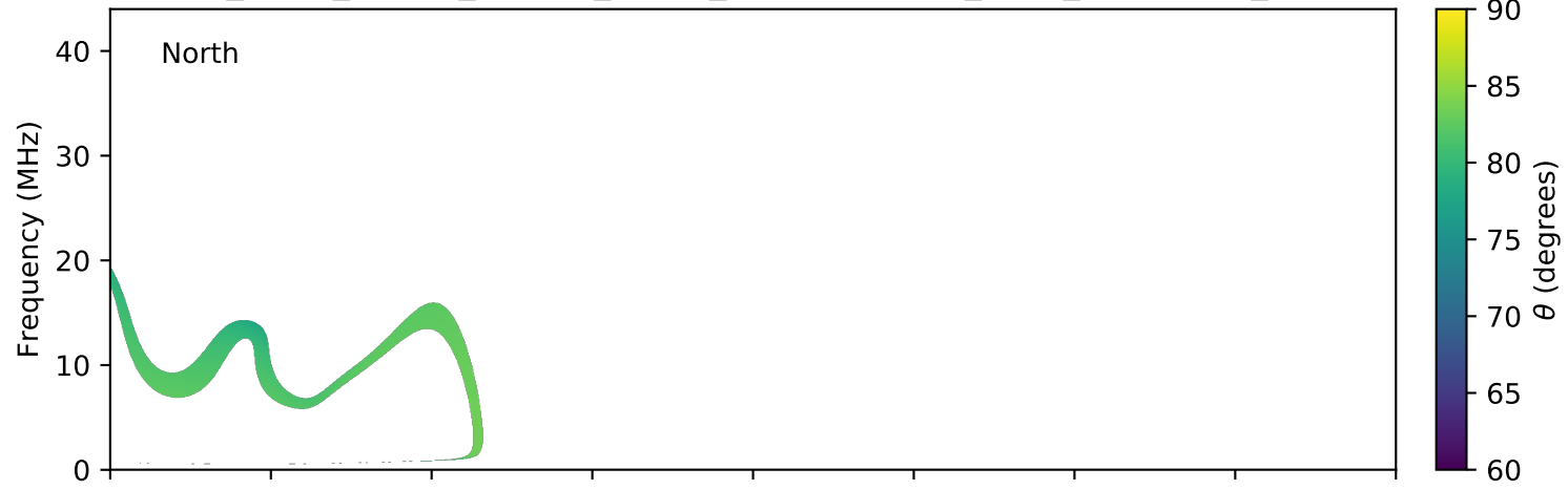
expres_earth_jupiter_europa_jrm09_lossc-wid1deg_3kev_20040919_v11.cdf
