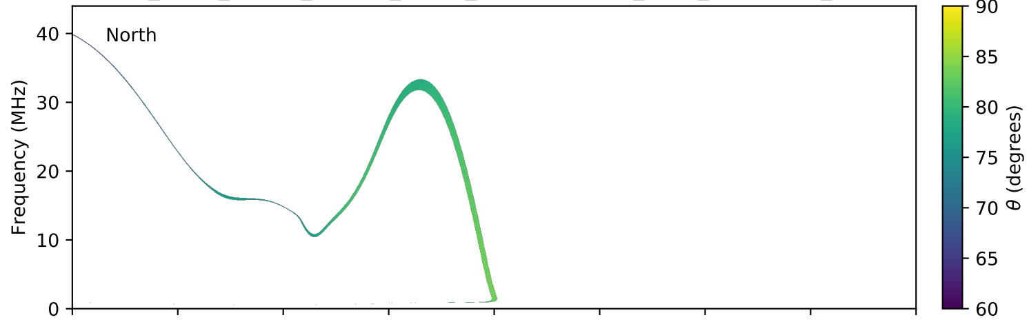
expres_earth_jupiter_europa_jrm09_lossc-wid1deg_3kev_20040918_v11.cdf
