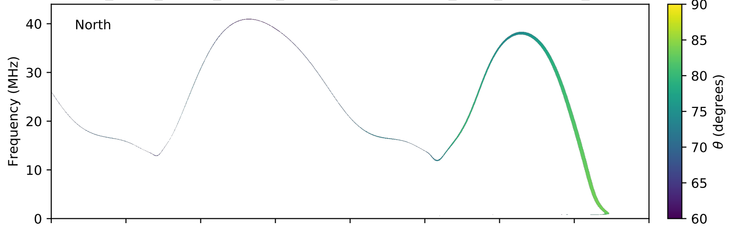
expres_earth_jupiter_europa_jrm09_lossc-wid1deg_3kev_20040904_v11.cdf
