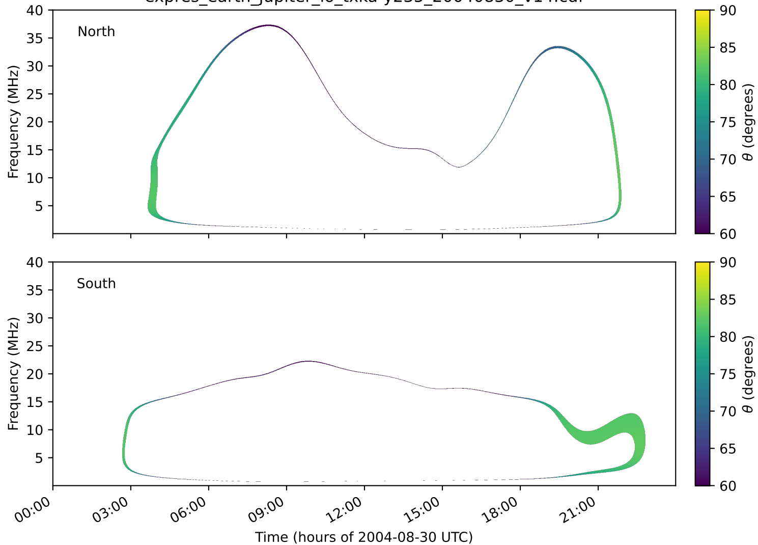
expres_earth_jupiter_io_txka-y235_20040830_v14.cdf
