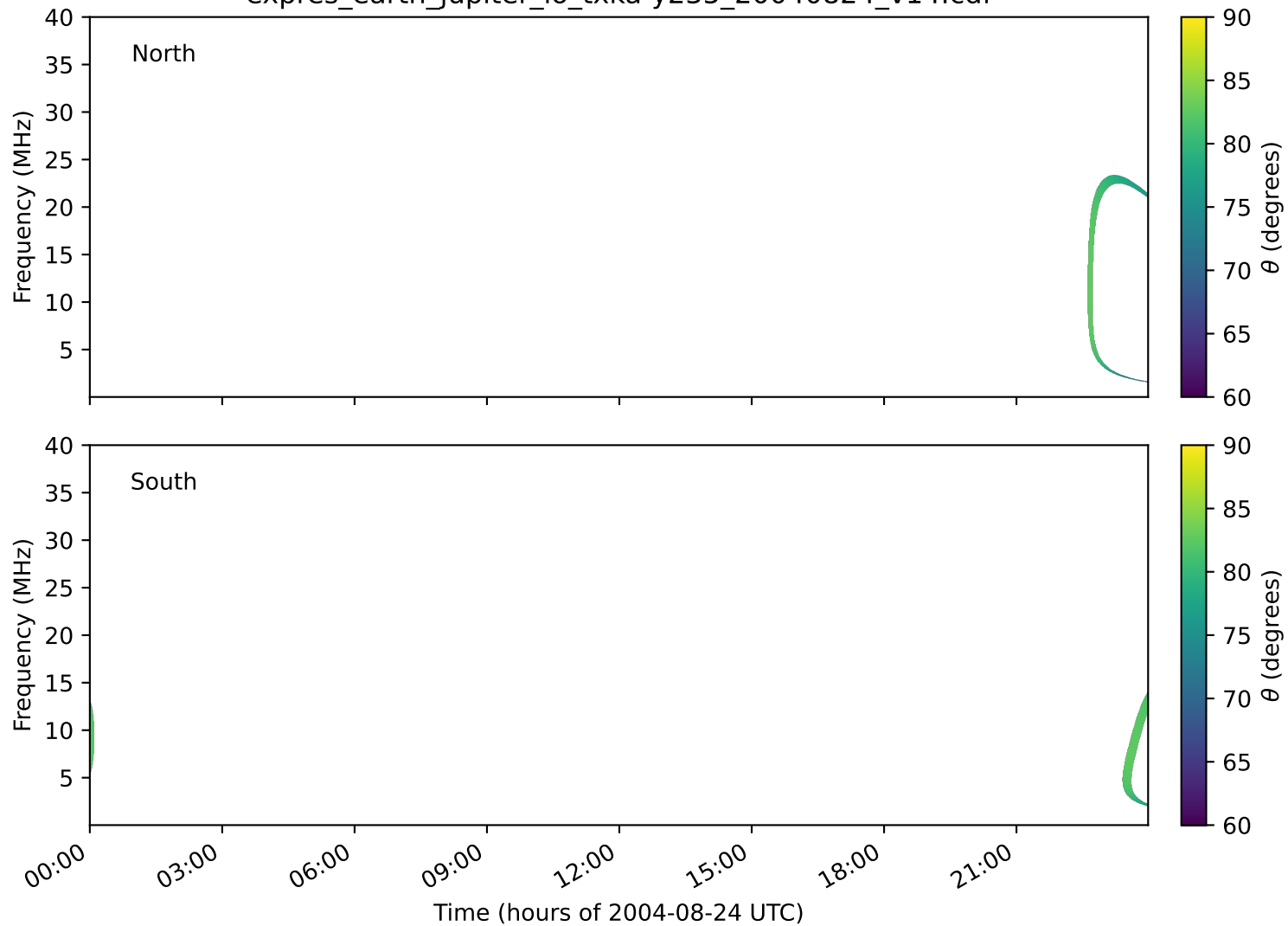
expres_earth_jupiter_io_txka-y235_20040824_v14.cdf
