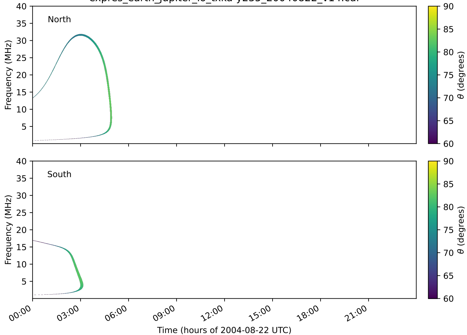
expres_earth_jupiter_io_txka-y235_20040822_v14.cdf
