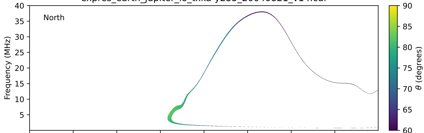
expres_earth_jupiter_io_txka-y235_20040821_v14.cdf
