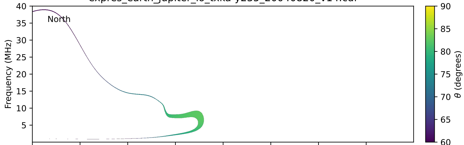
expres_earth_jupiter_io_txka-y235_20040820_v14.cdf
