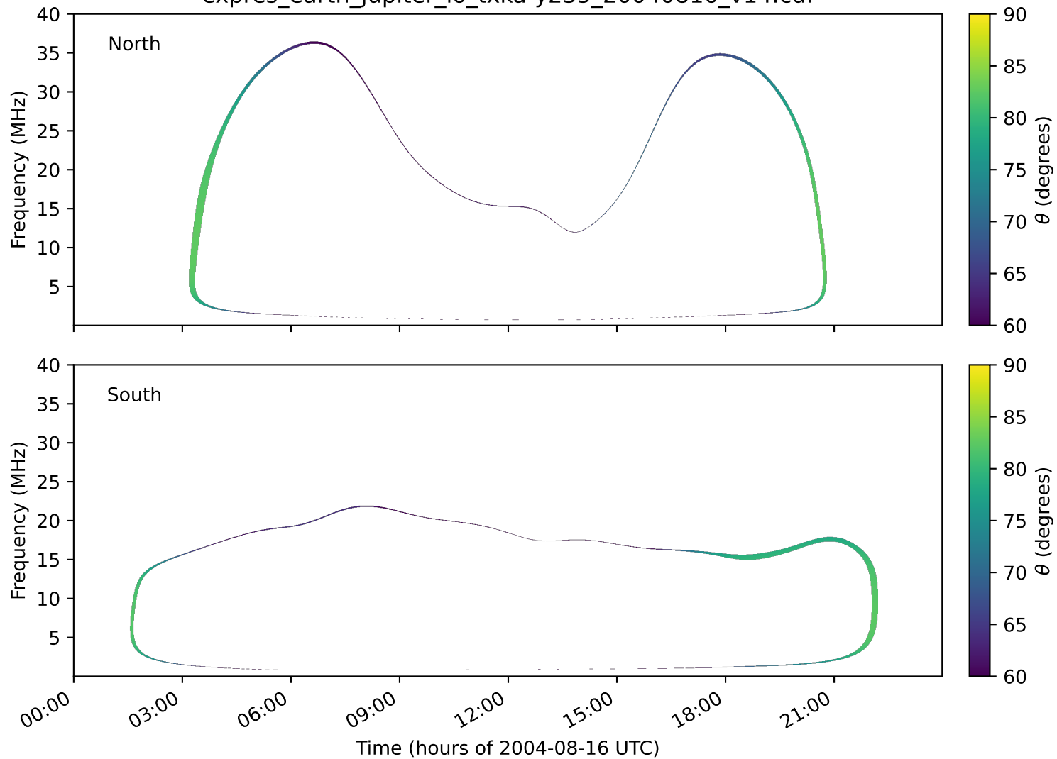
expres_earth_jupiter_io_txka-y235_20040816_v14.cdf
