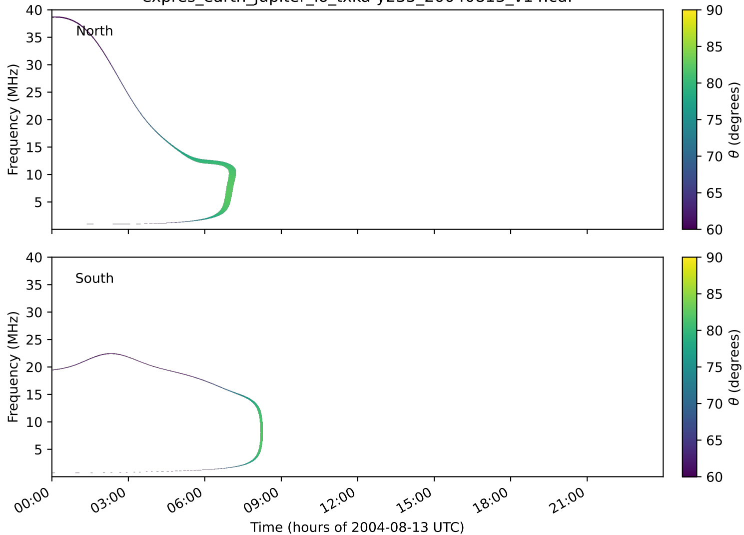
expres_earth_jupiter_io_txka-y235_20040813_v14.cdf
