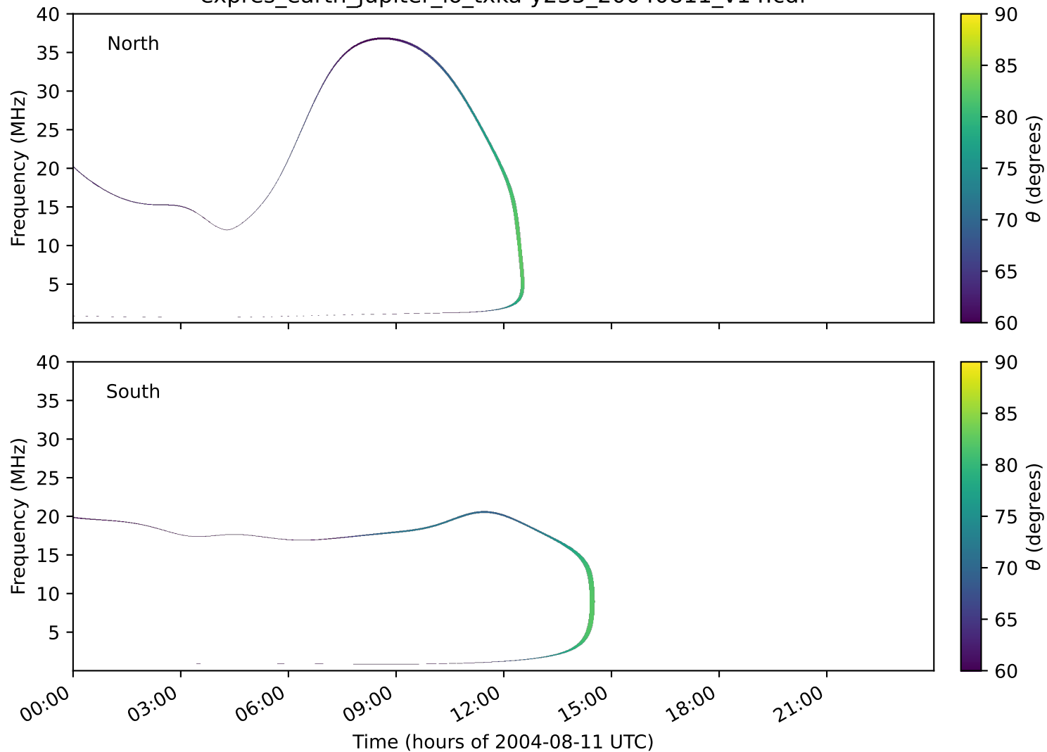
expres_earth_jupiter_io_txka-y235_20040811_v14.cdf
