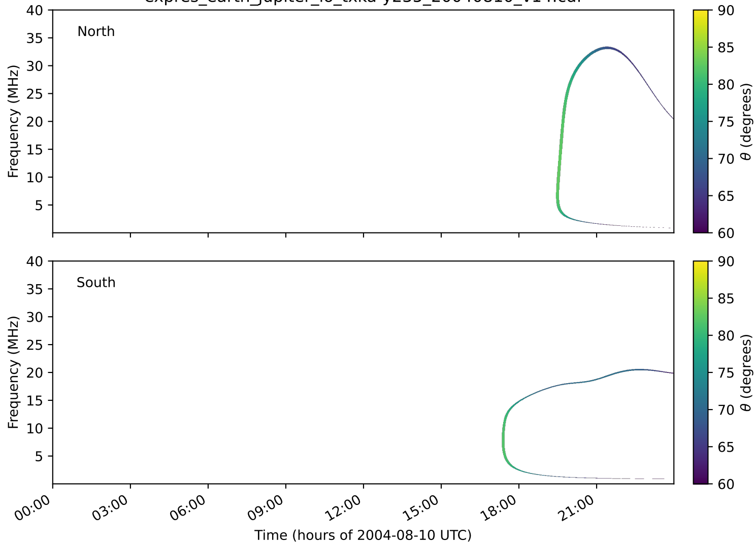
expres_earth_jupiter_io_txka-y235_20040810_v14.cdf
