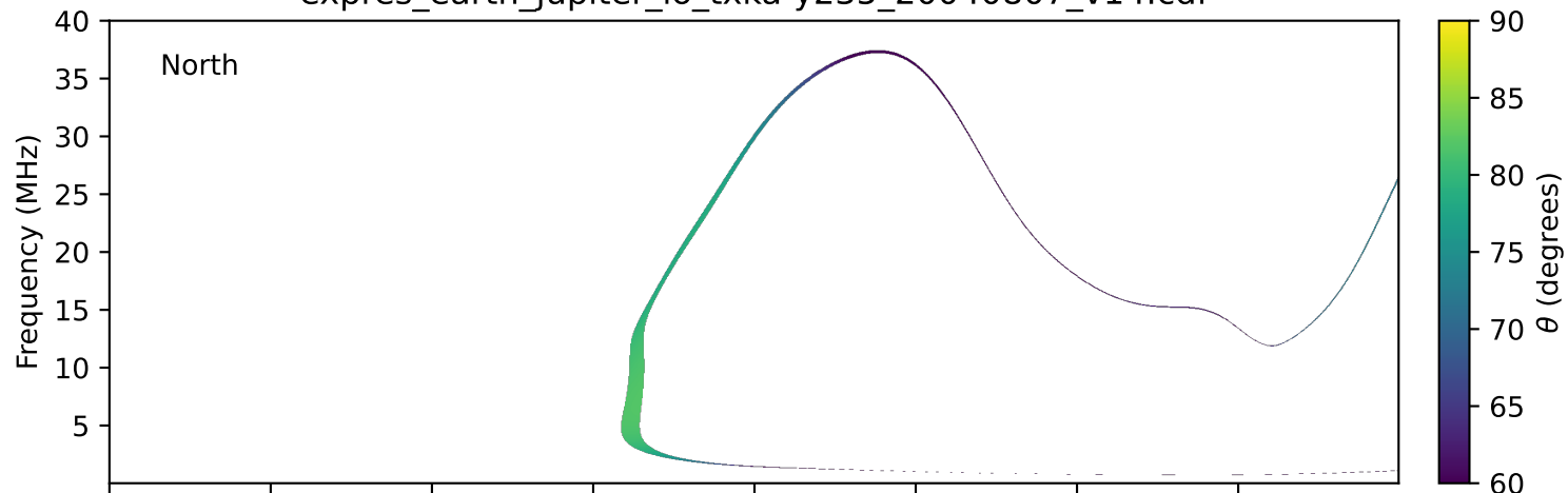
expres_earth_jupiter_io_txka-y235_20040807_v14.cdf
