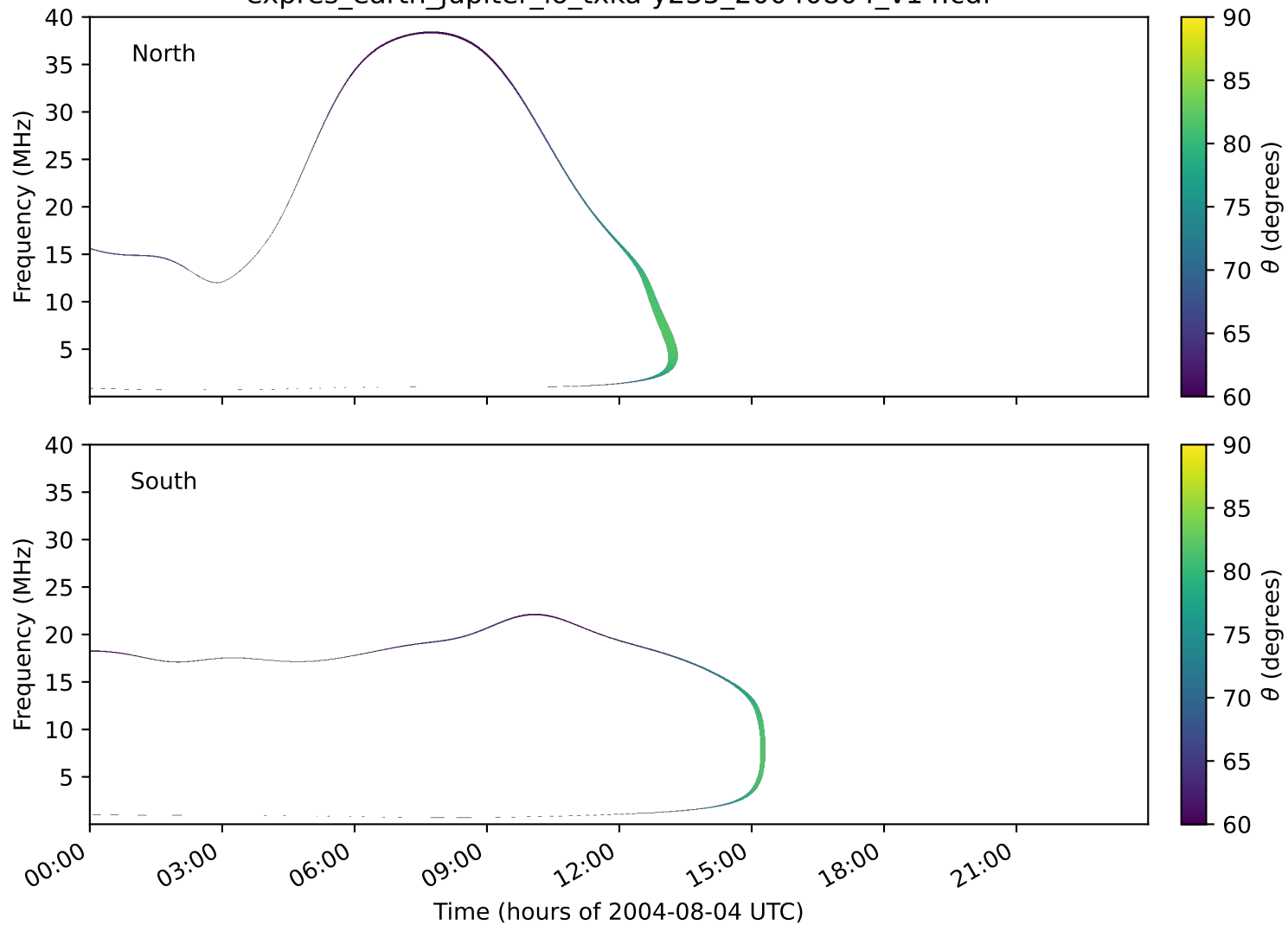
expres_earth_jupiter_io_txka-y235_20040804_v14.cdf
