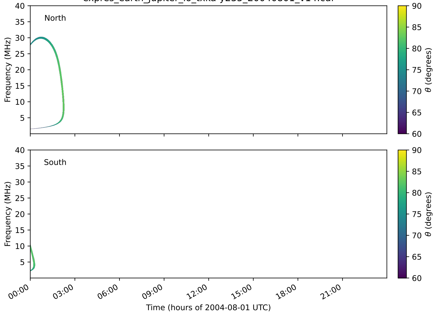
expres_earth_jupiter_io_txka-y235_20040801_v14.cdf
