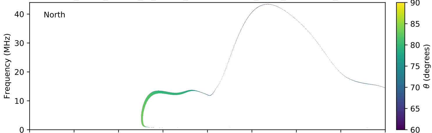
expres_earth_jupiter_io_jrm09_lossc-wid1deg_3kev_20040828_v11.cdf
