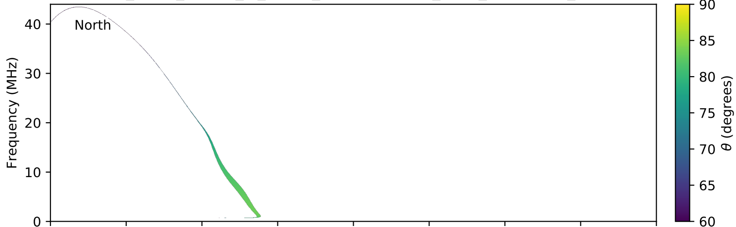
expres_earth_jupiter_io_jrm09_lossc-wid1deg_3kev_20040827_v11.cdf
