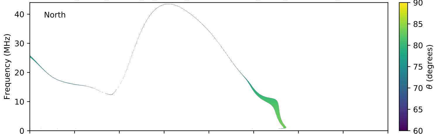
expres_earth_jupiter_io_jrm09_lossc-wid1deg_3kev_20040825_v11.cdf
