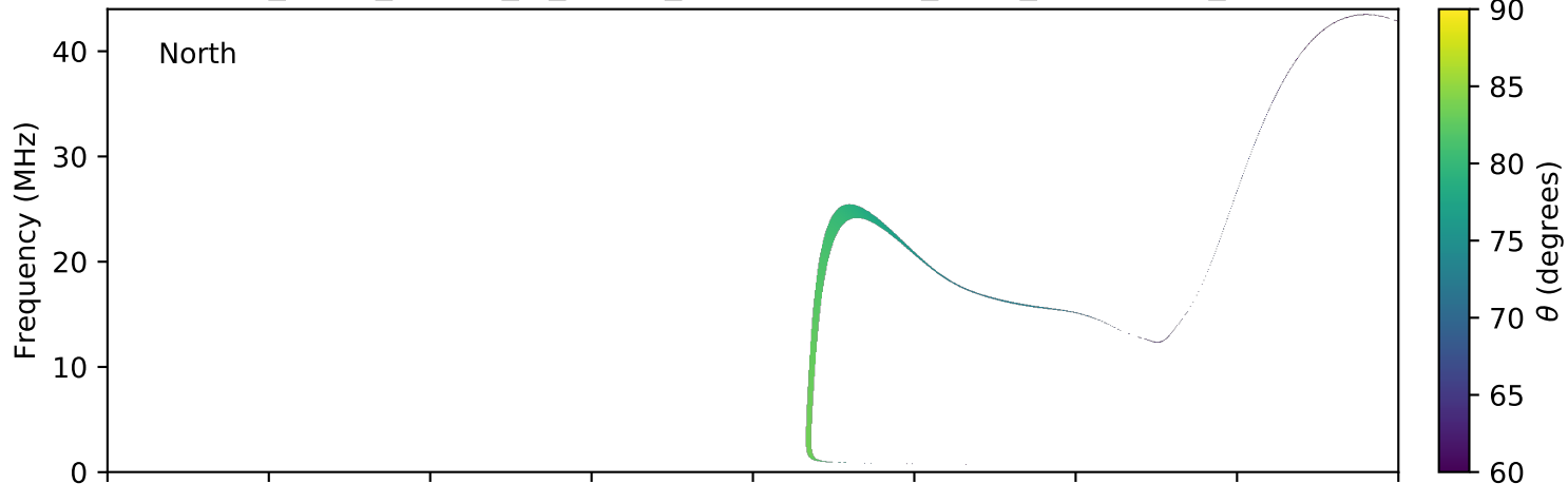
expres_earth_jupiter_io_jrm09_lossc-wid1deg_3kev_20040812_v11.cdf
