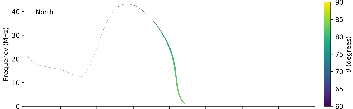
expres_earth_jupiter_io_jrm09_lossc-wid1deg_3kev_20040811_v11.cdf
