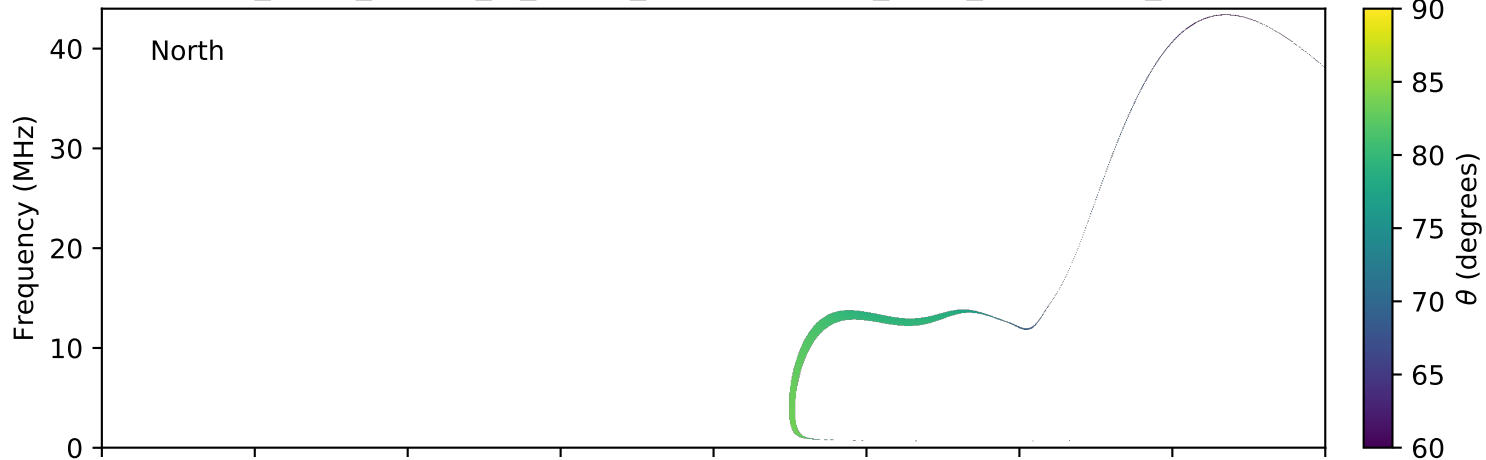
expres_earth_jupiter_io_jrm09_lossc-wid1deg_3kev_20040805_v11.cdf
