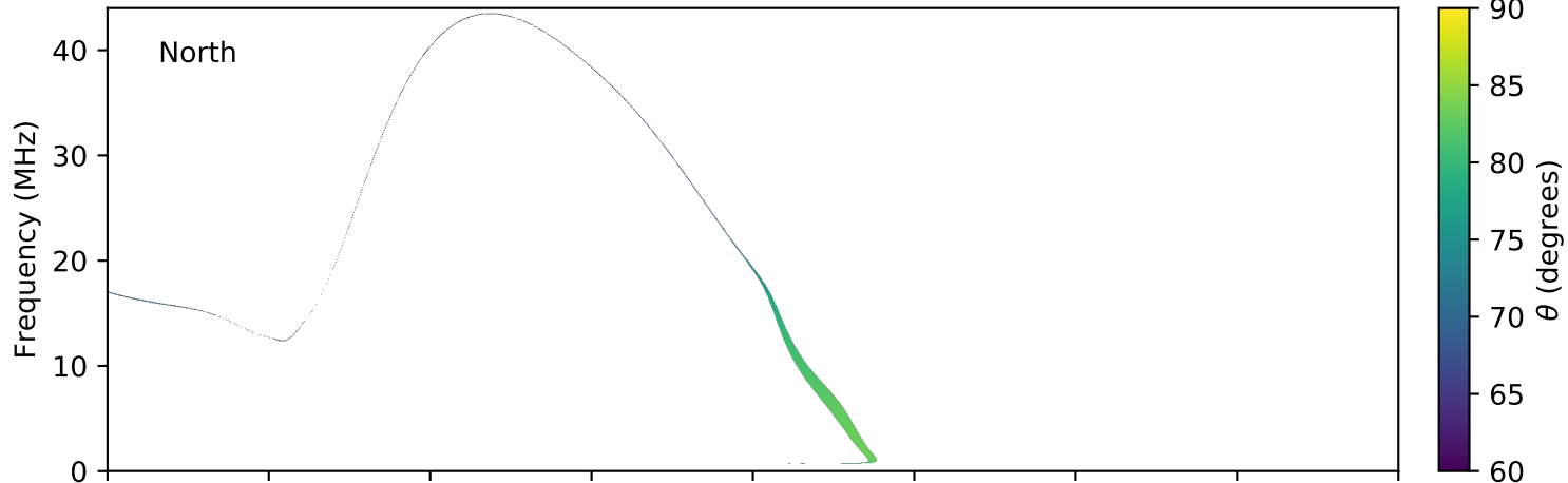
expres_earth_jupiter_io_jrm09_lossc-wid1deg_3kev_20040804_v11.cdf
