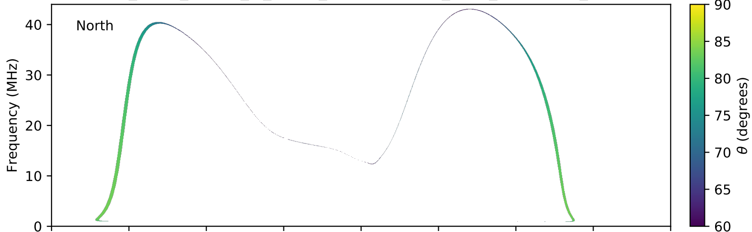
expres_earth_jupiter_io_jrm09_lossc-wid1deg_3kev_20040802_v11.cdf
