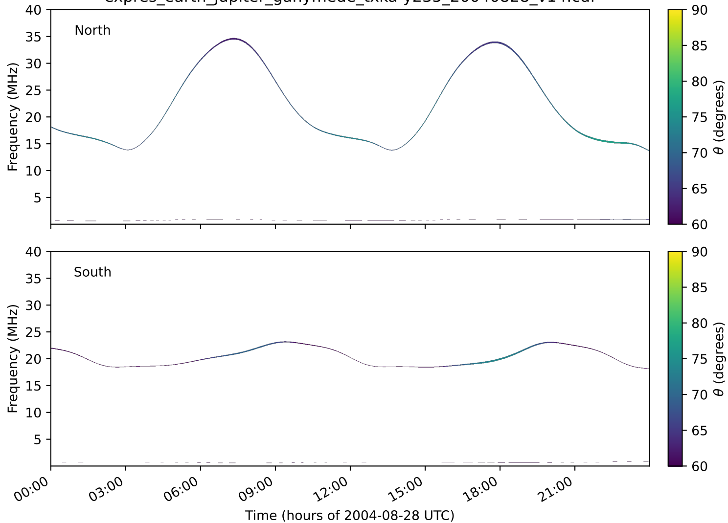
expres_earth_jupiter_ganymede_txka-y235_20040828_v14.cdf
