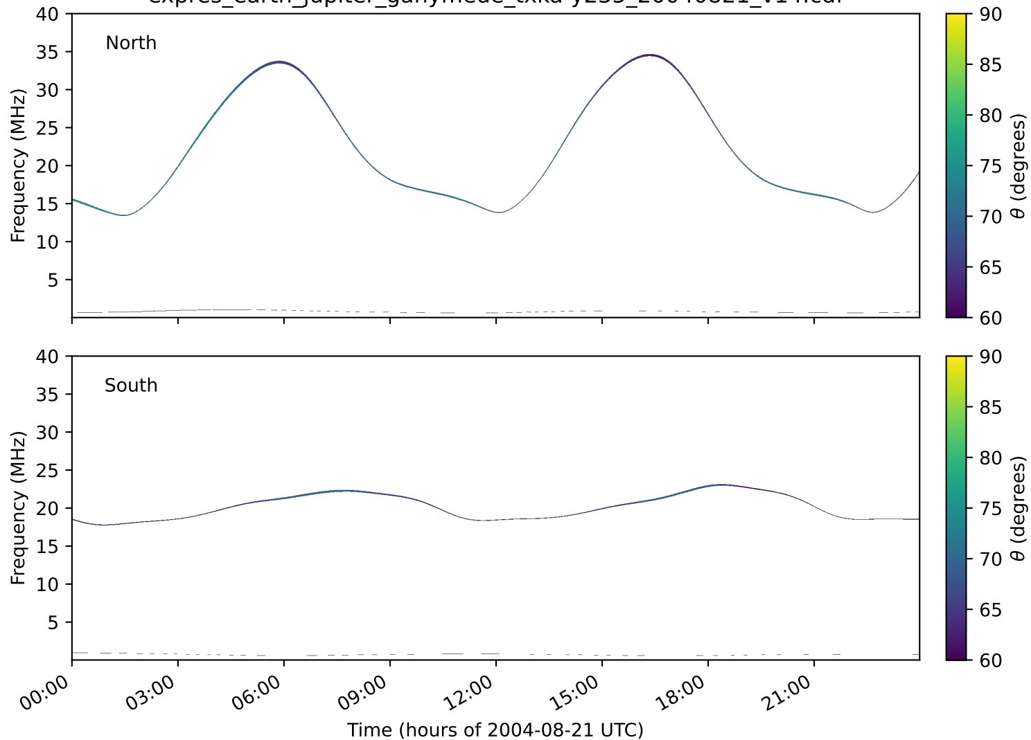
expres_earth_jupiter_ganymede_txka-y235_20040821_v14.cdf
