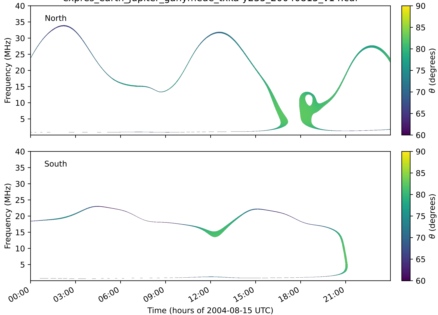
expres_earth_jupiter_ganymede_txka-y235_20040815_v14.cdf
