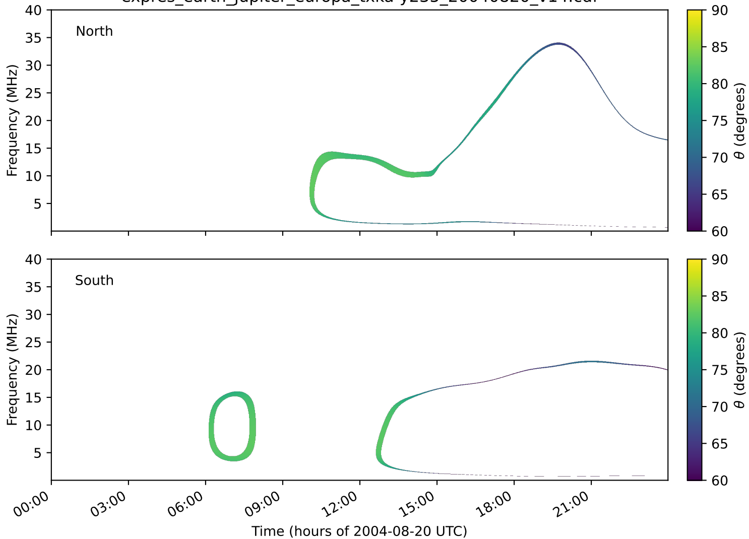
expres_earth_jupiter_europa_txka-y235_20040820_v14.cdf
