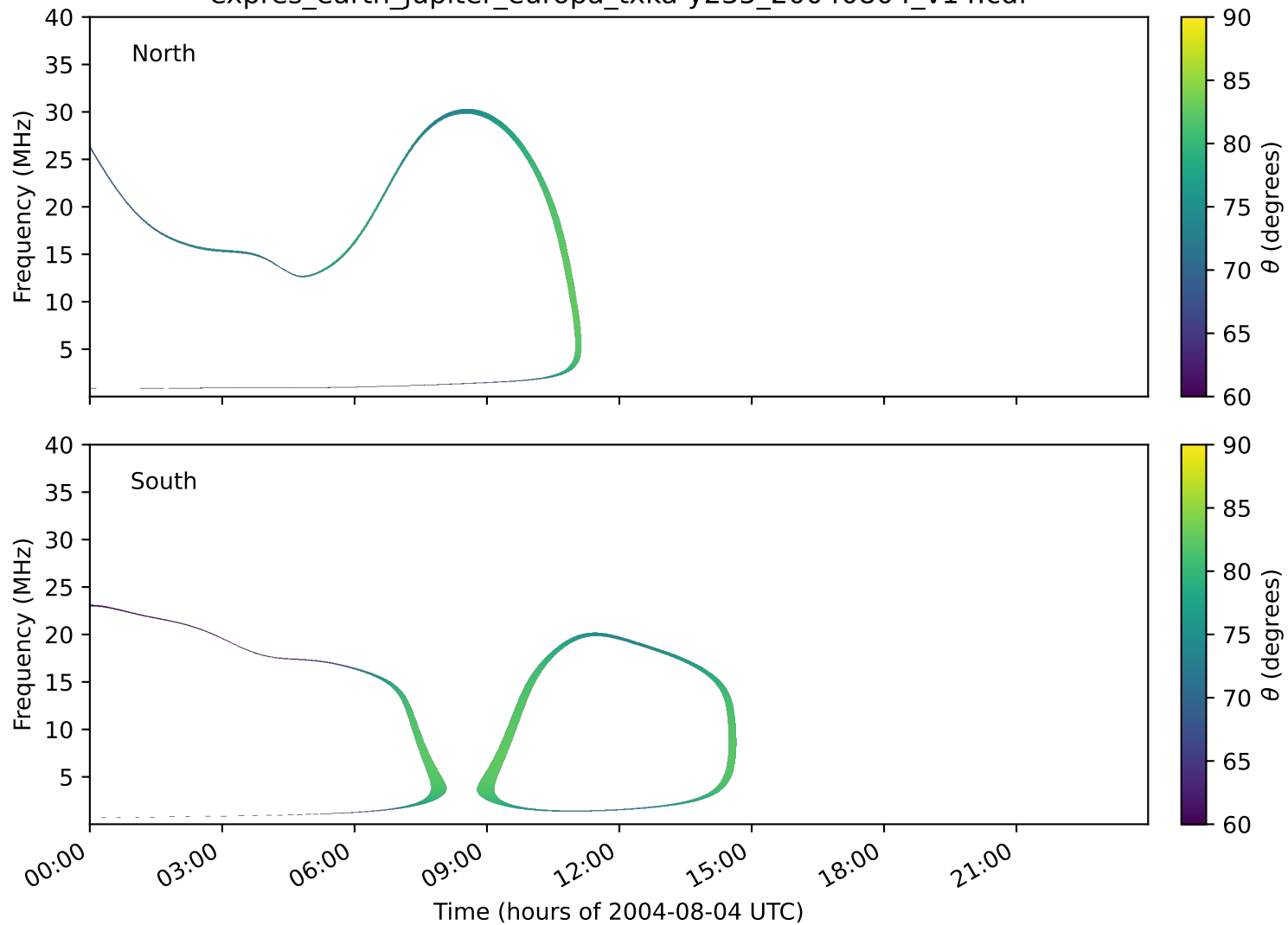
expres_earth_jupiter_europa_txka-y235_20040804_v14.cdf
