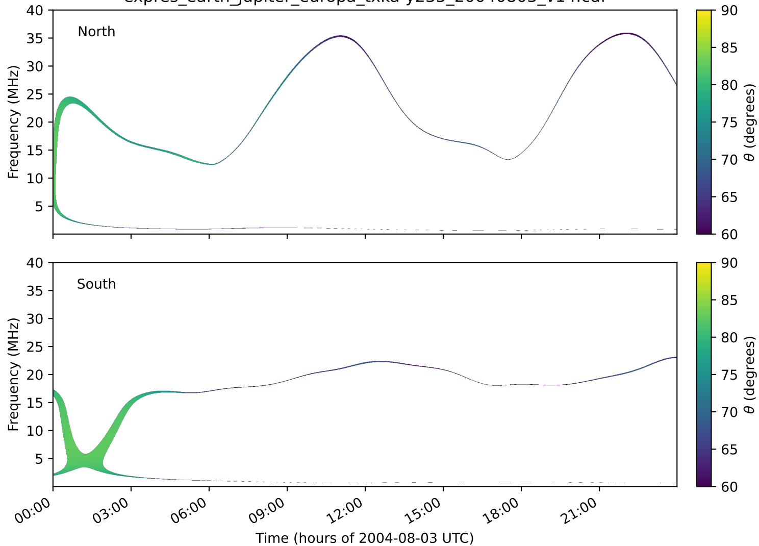
expres_earth_jupiter_europa_txka-y235_20040803_v14.cdf
