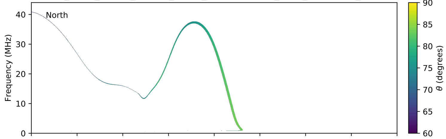
expres_earth_jupiter_europa_jrm09_lossc-wid1deg_3kev_20040825_v11.cdf
