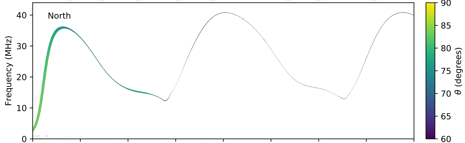
expres_earth_jupiter_europa_jrm09_lossc-wid1deg_3kev_20040817_v11.cdf
