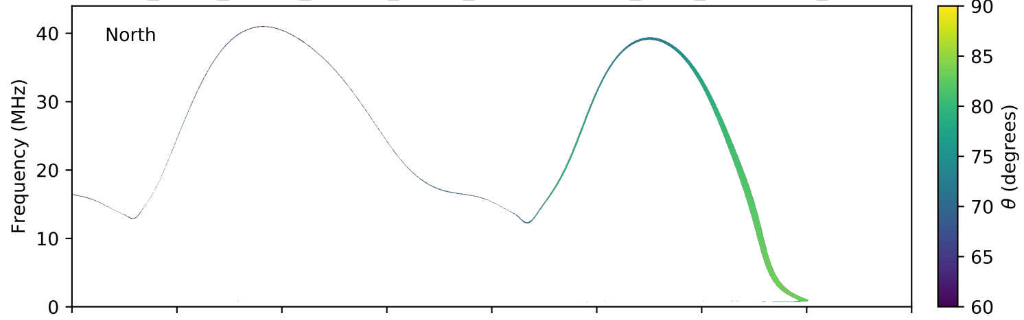
expres_earth_jupiter_europa_jrm09_lossc-wid1deg_3kev_20040814_v11.cdf
