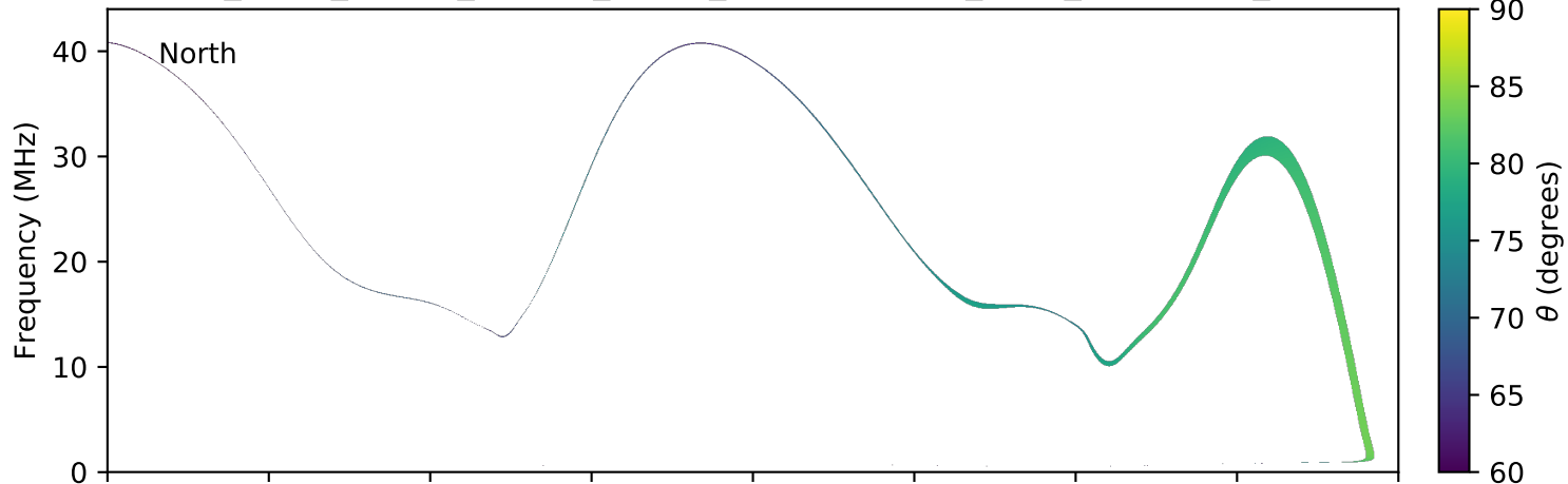
expres_earth_jupiter_europa_jrm09_lossc-wid1deg_3kev_20040808_v11.cdf
