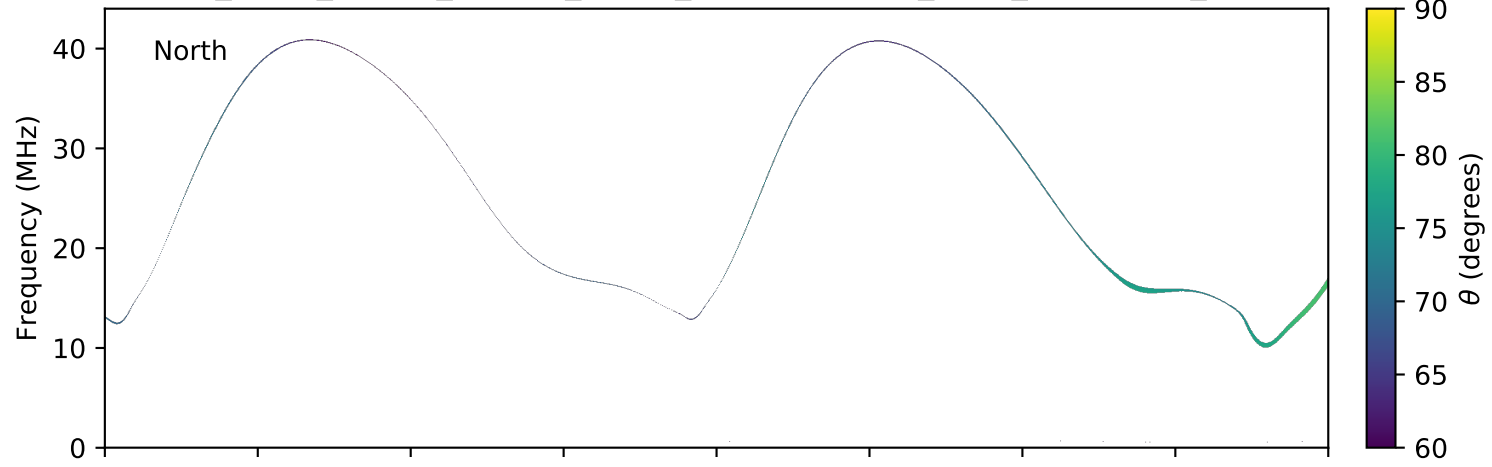
expres_earth_jupiter_europa_jrm09_lossc-wid1deg_3kev_20040807_v11.cdf
