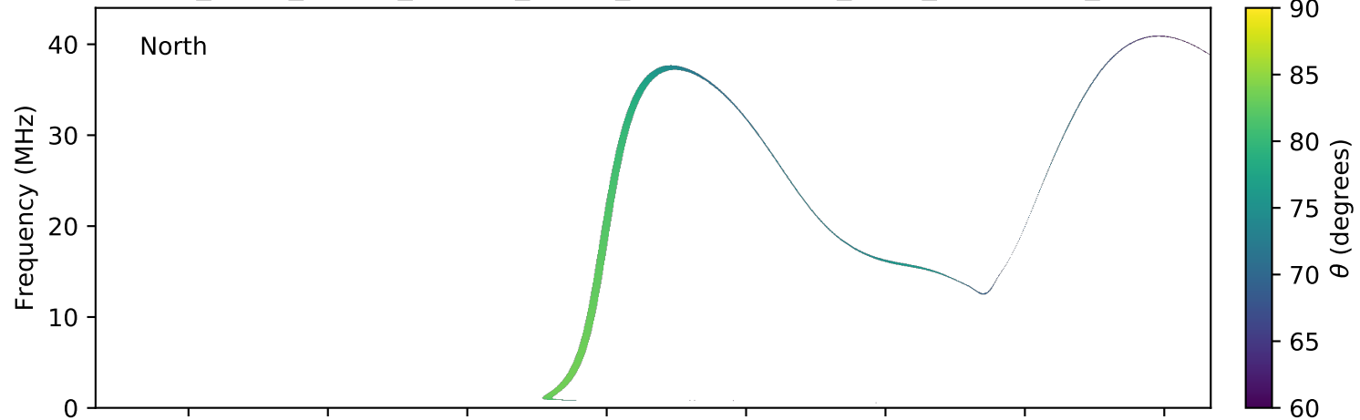
expres_earth_jupiter_europa_jrm09_lossc-wid1deg_3kev_20040800_v11.cdf
