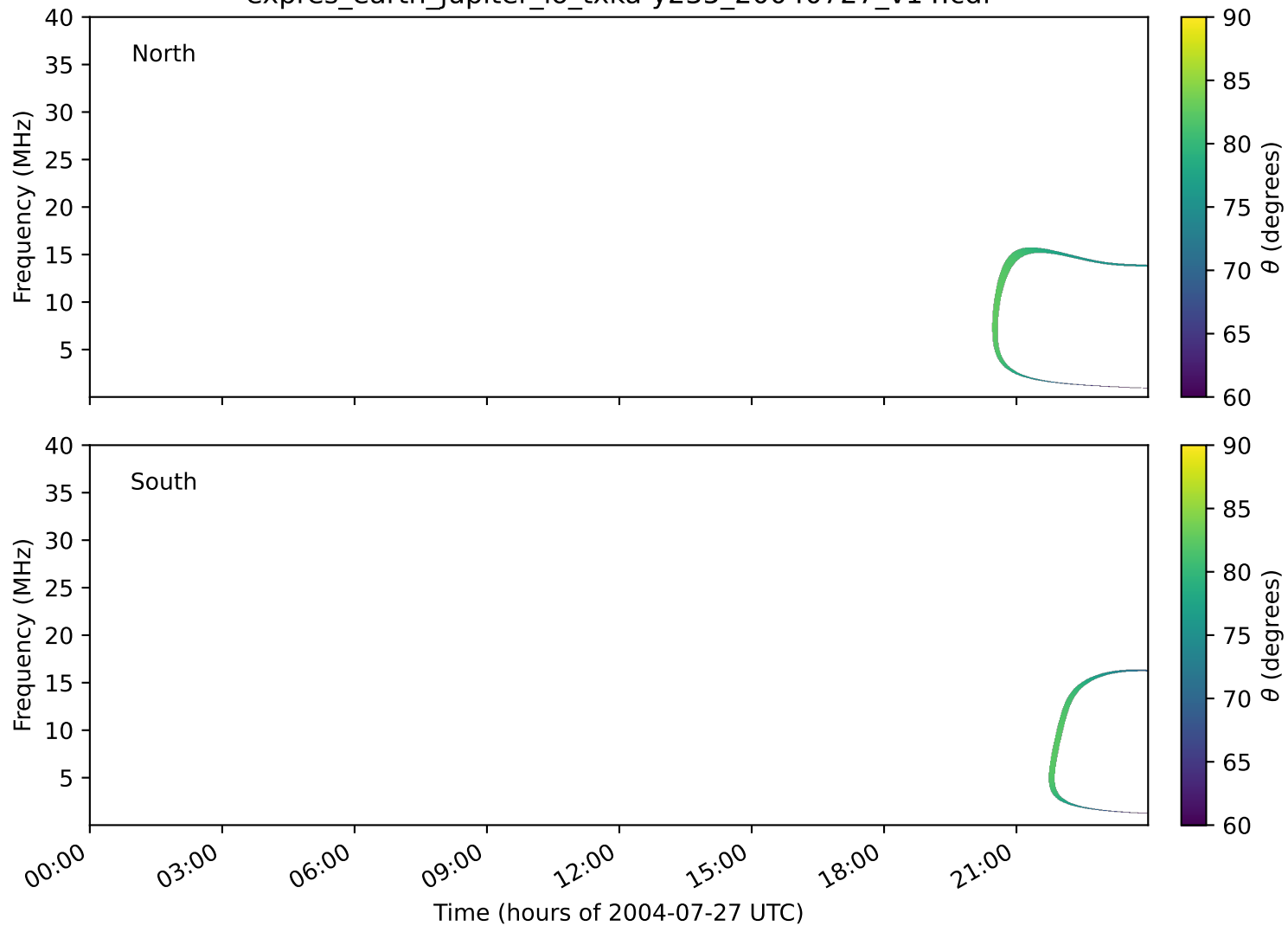
expres_earth_jupiter_io_txka-y235_20040727_v14.cdf
