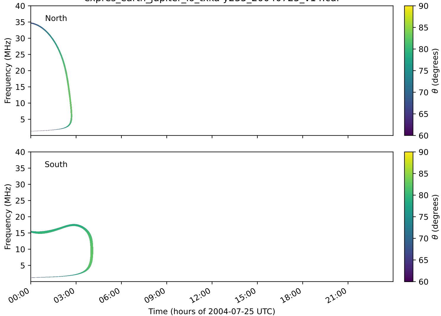
expres_earth_jupiter_io_txka-y235_20040725_v14.cdf
