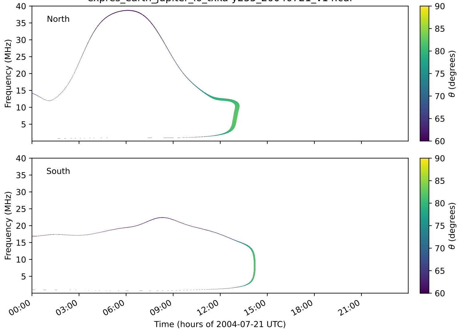
expres_earth_jupiter_io_txka-y235_20040721_v14.cdf
