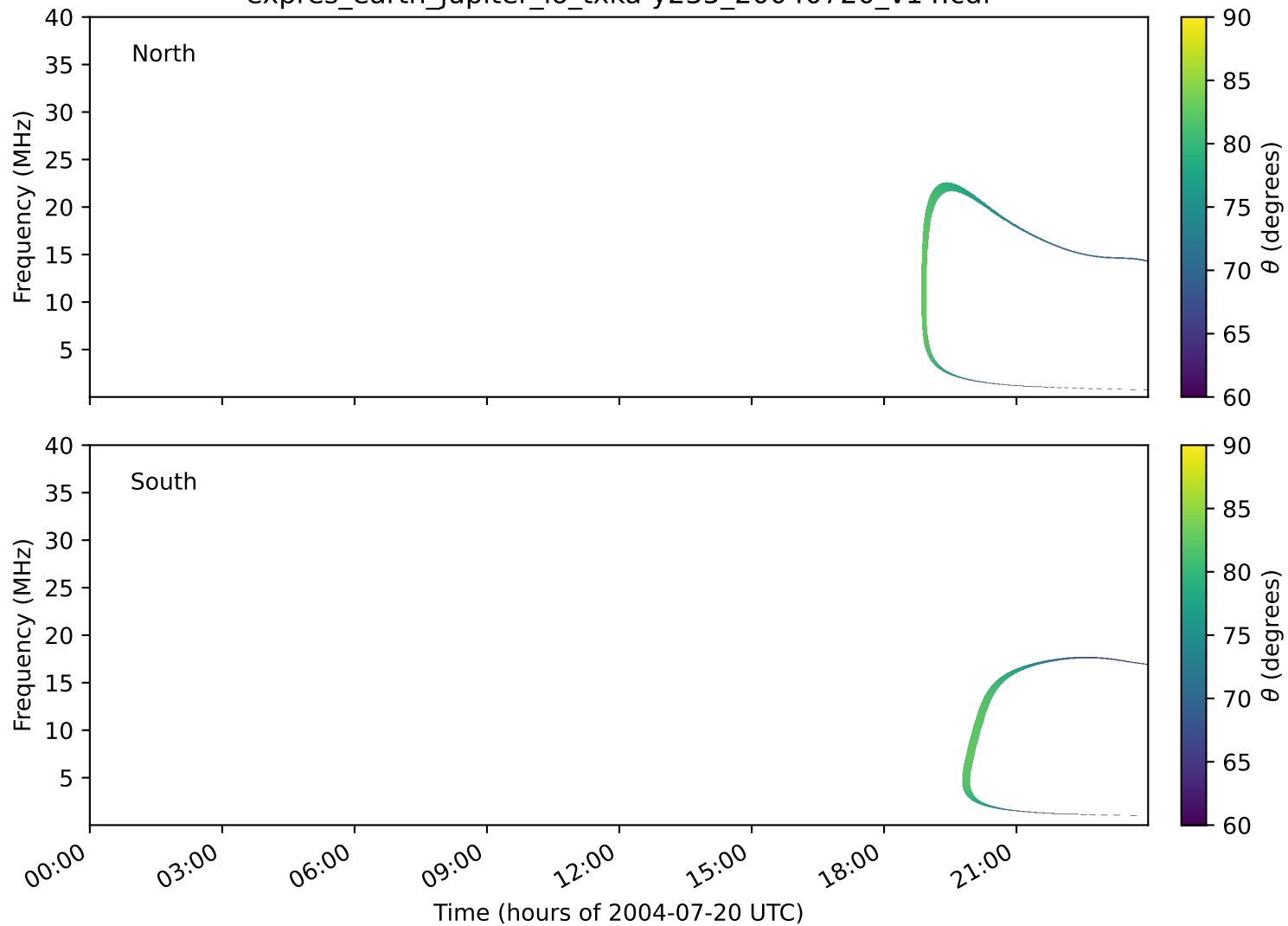
expres_earth_jupiter_io_txka-y235_20040720_v14.cdf
