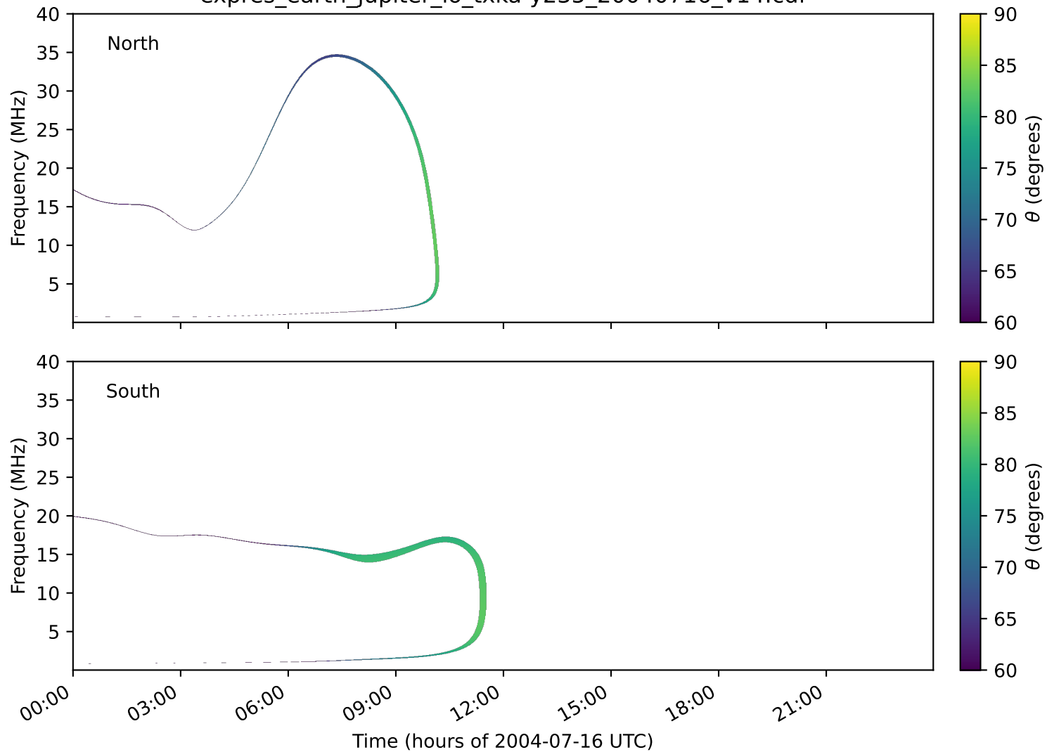
expres_earth_jupiter_io_txka-y235_20040716_v14.cdf
