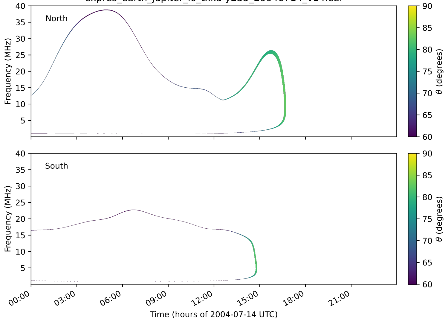
expres_earth_jupiter_io_txka-y235_20040714_v14.cdf
