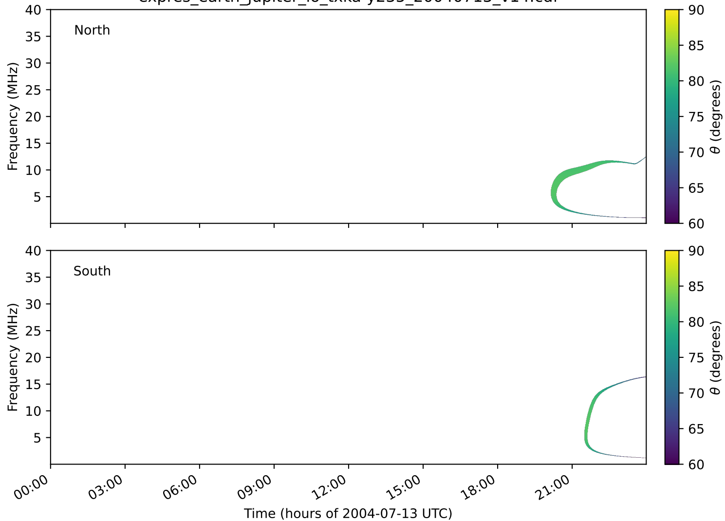
expres_earth_jupiter_io_txka-y235_20040713_v14.cdf
