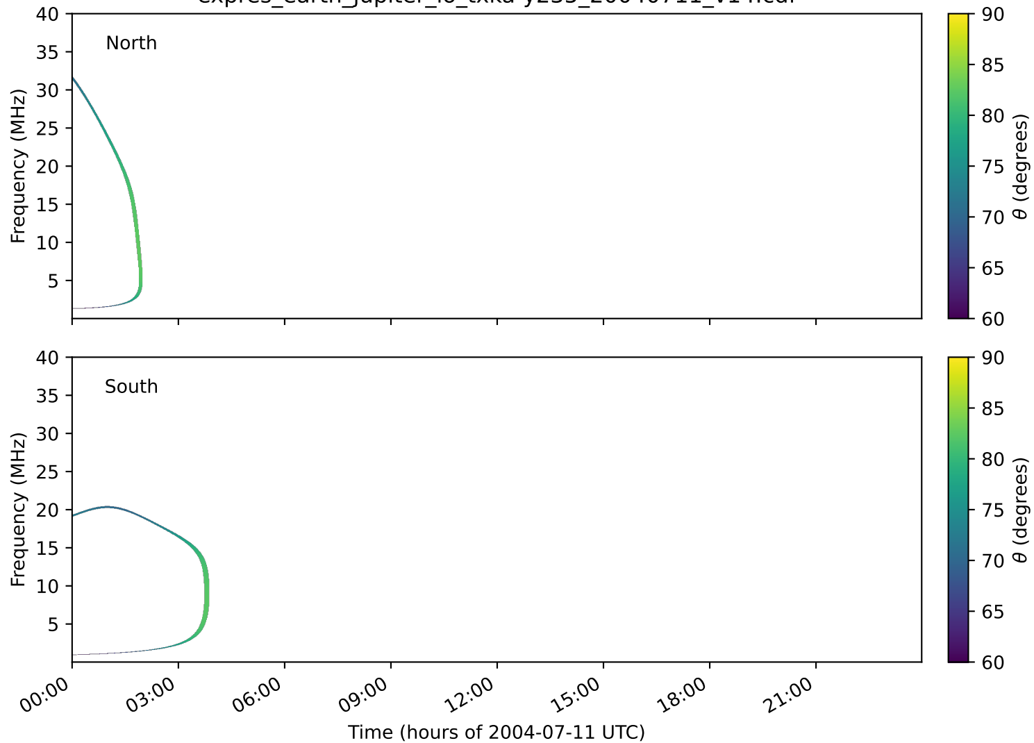
expres_earth_jupiter_io_txka-y235_20040711_v14.cdf
