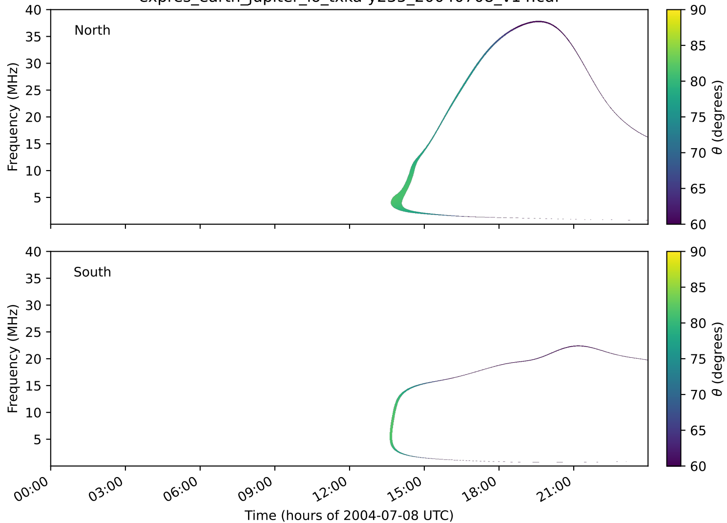
expres_earth_jupiter_io_txka-y235_20040708_v14.cdf
