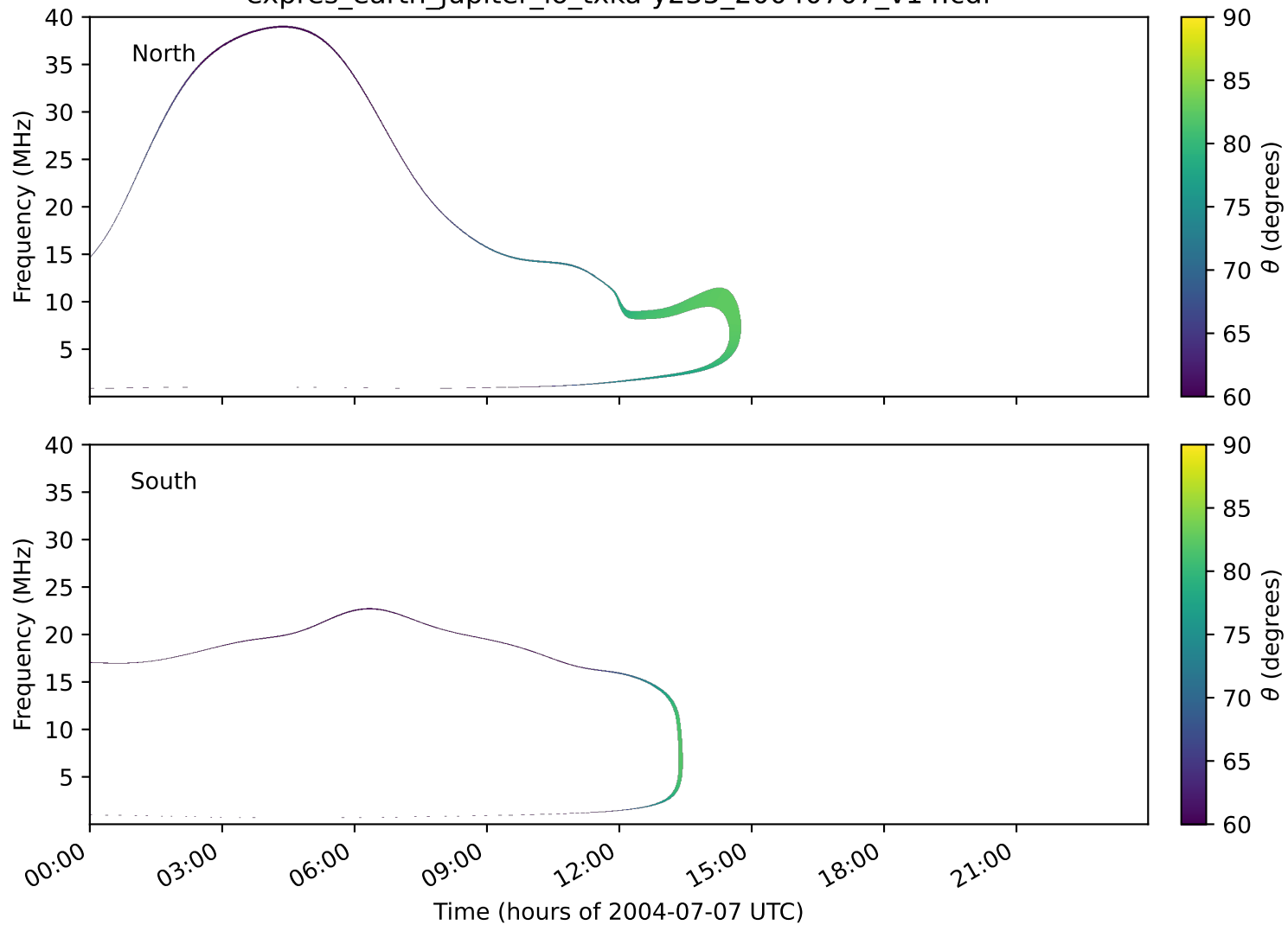
expres_earth_jupiter_io_txka-y235_20040707_v14.cdf
