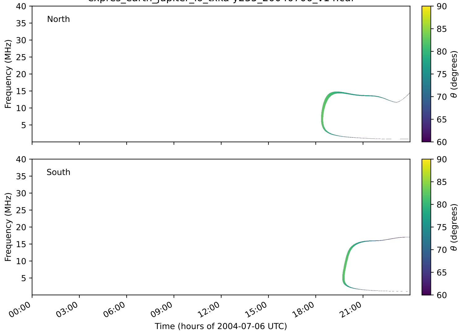
expres_earth_jupiter_io_txka-y235_20040706_v14.cdf
