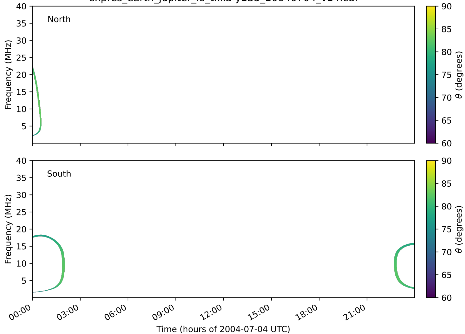
expres_earth_jupiter_io_txka-y235_20040704_v14.cdf
