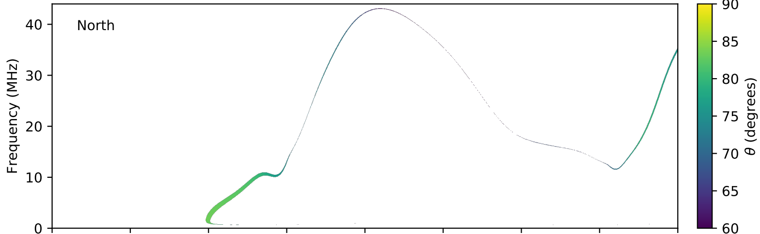
expres_earth_jupiter_io_jrm09_lossc-wid1deg_3kev_20040731_v11.cdf
