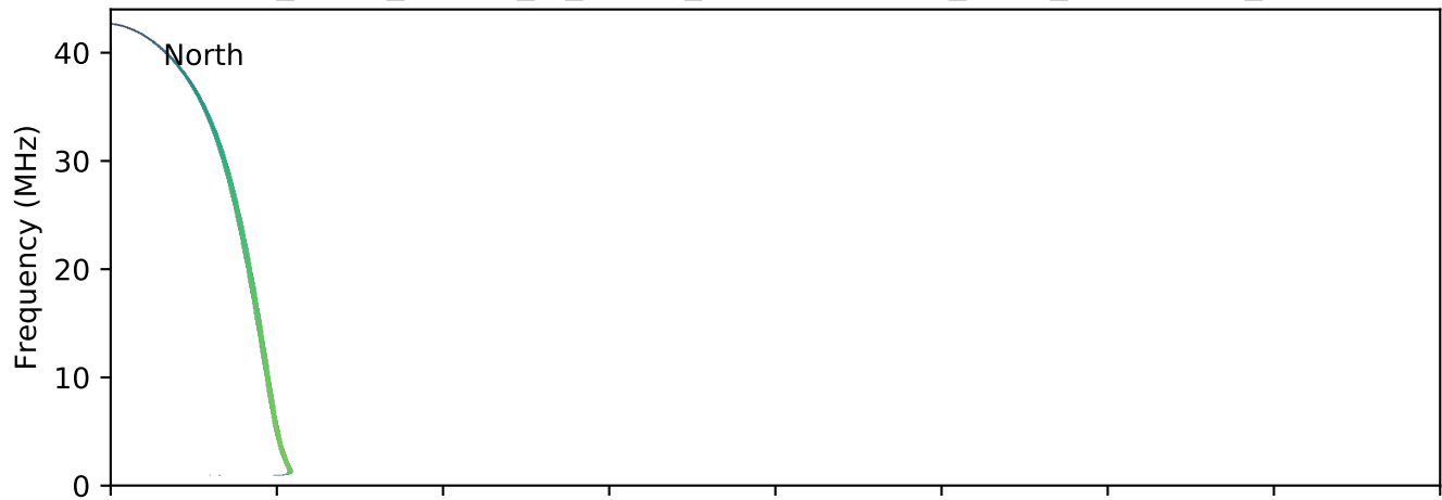
expres_earth_jupiter_io_jrm09_lossc-wid1deg_3kev_20040725_v11.cdf
