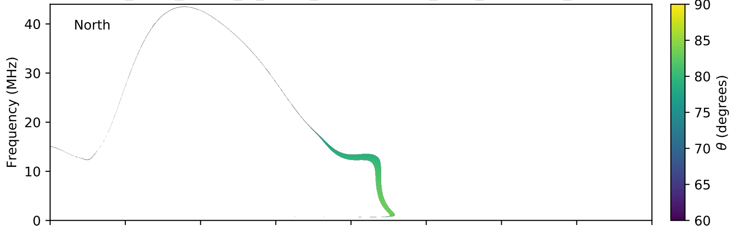
expres_earth_jupiter_io_jrm09_lossc-wid1deg_3kev_20040721_v11.cdf
